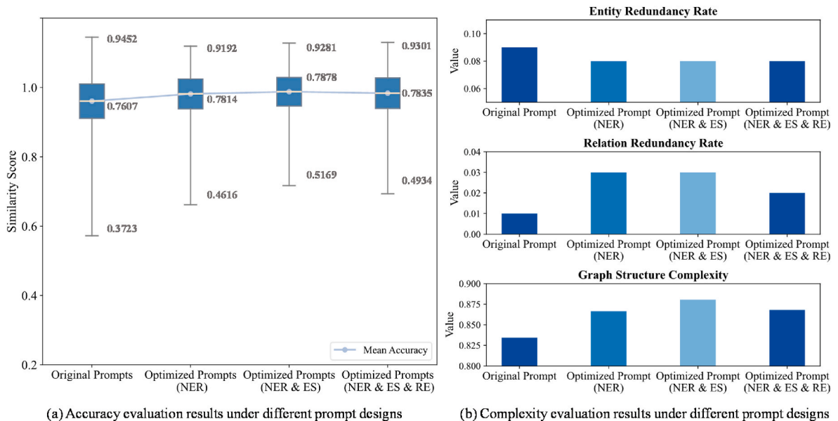
Fig. 7. KG Quality evaluation across varying prompt designs: original prompts, optimized prompt for NER, optimized prompt for entity standardization (ES), optimized prompt for relation extraction (RE). In each step, one more prompt is optimized in order.
