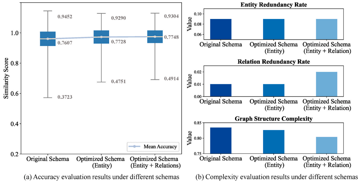
Fig. 6. KG Quality evaluation across varying schema designs: original schema, schema with optimized entity type definitions, and schema with optimized relation type definitions.
