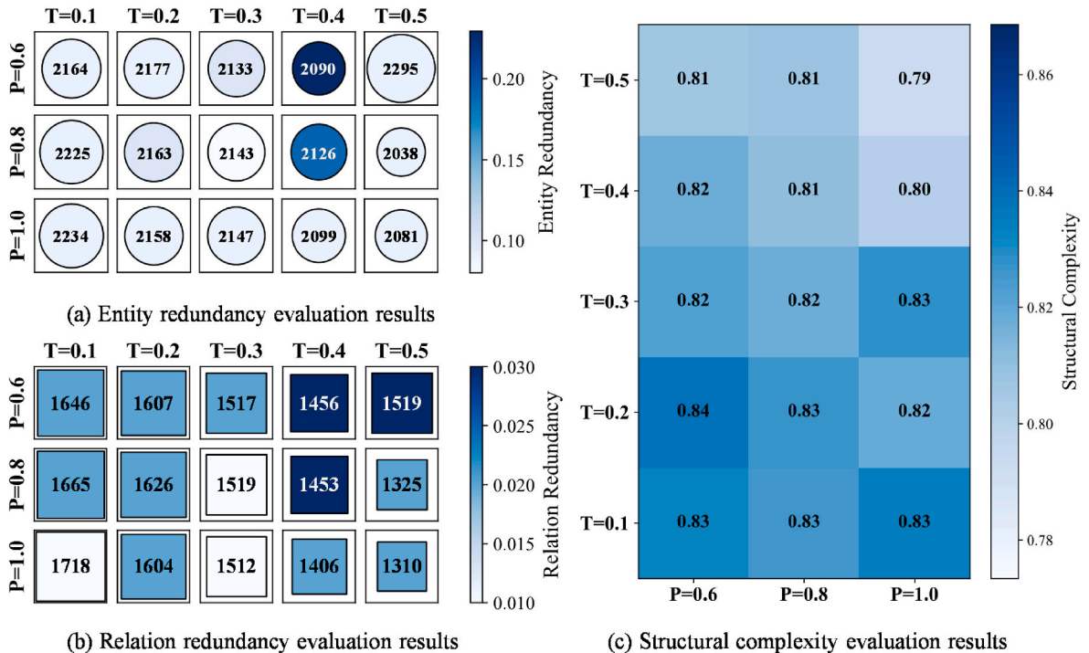
Fig. 5. Complexity evaluation of entities, relations, and graph structure under varying LLM decoding parameters (temperature, denoted as T, and Top- p , denoted as P) on the MAIB corpus.
